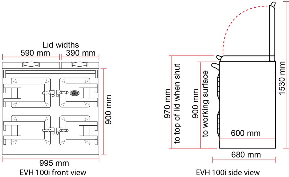
EVH100i dimensions
