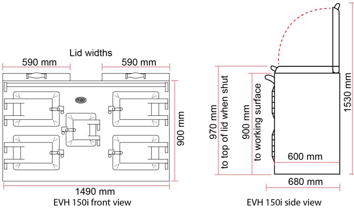
EVH150i dimensions
