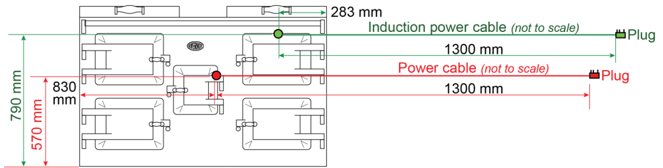
EVH 150i cable lengths
