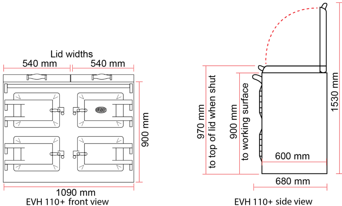
EVH110+ dimensions
