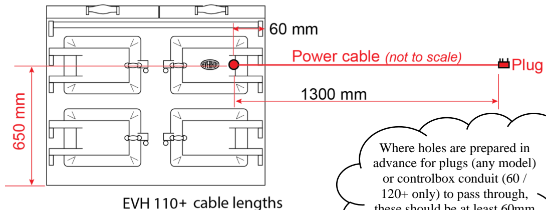
EVH110+ dimensions
