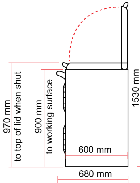
EVH 90 Plus side view
