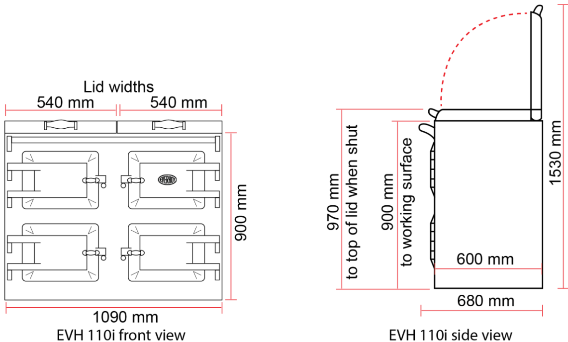
EVH110i dimensions
