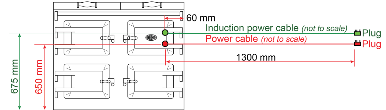
EVH110i dimensions
