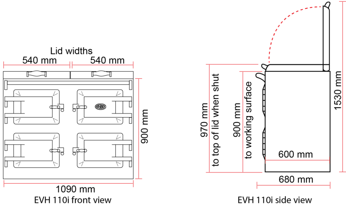
EVH110i dimensions
