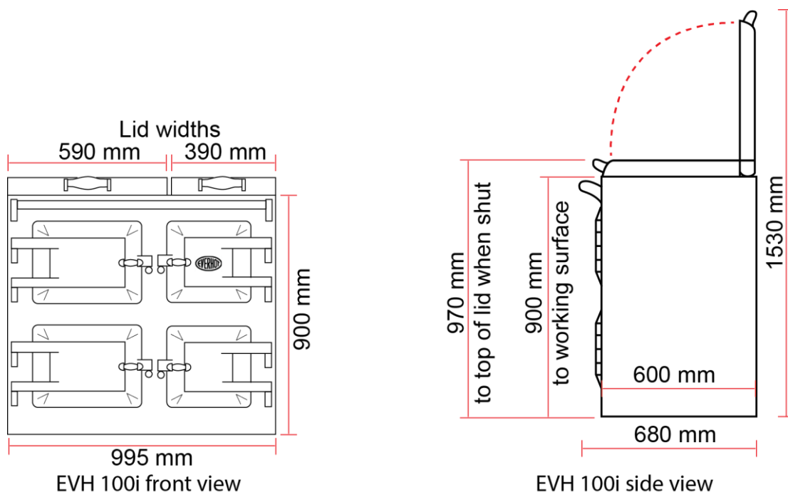
EVH100i dimensions
