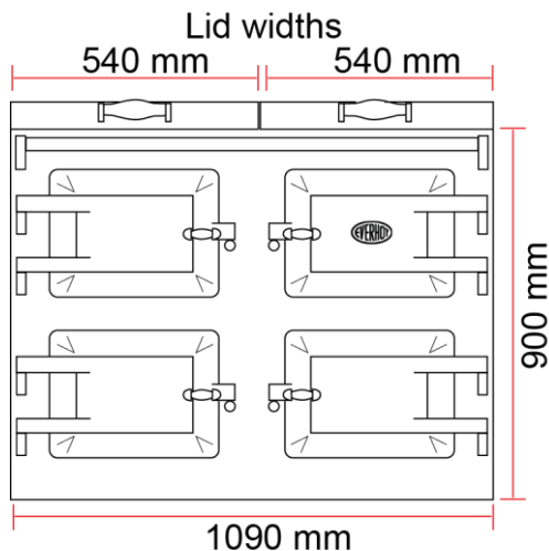
EVH 110i front view
