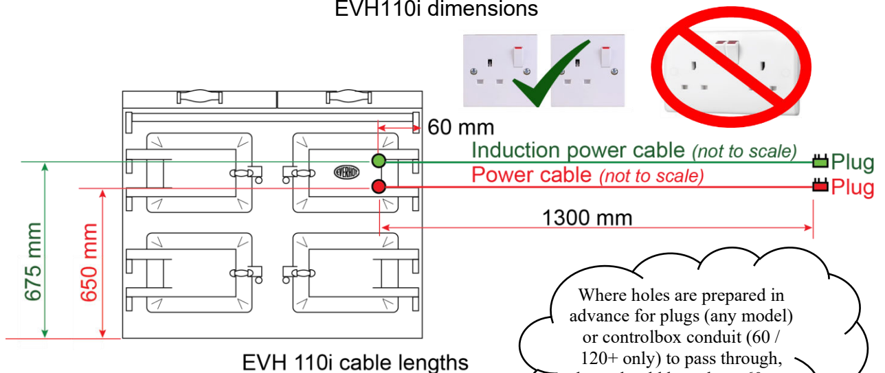
EVH110i dimensions
