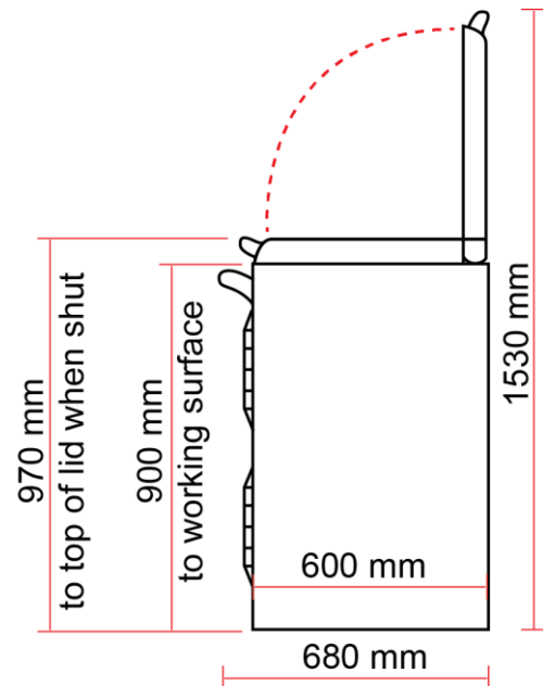
EVH 110i side view
