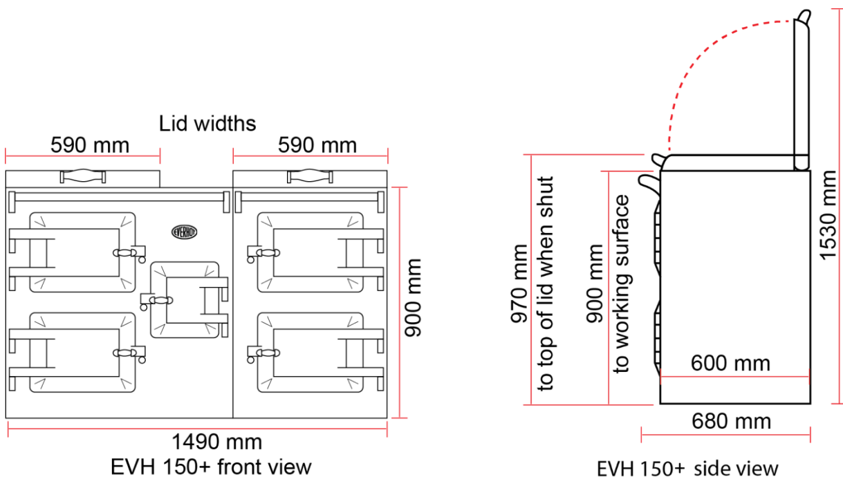
EVH150+ dimensions
