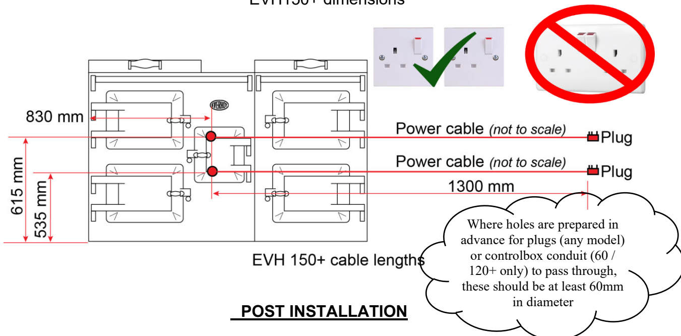
EVH150+ dimensions
