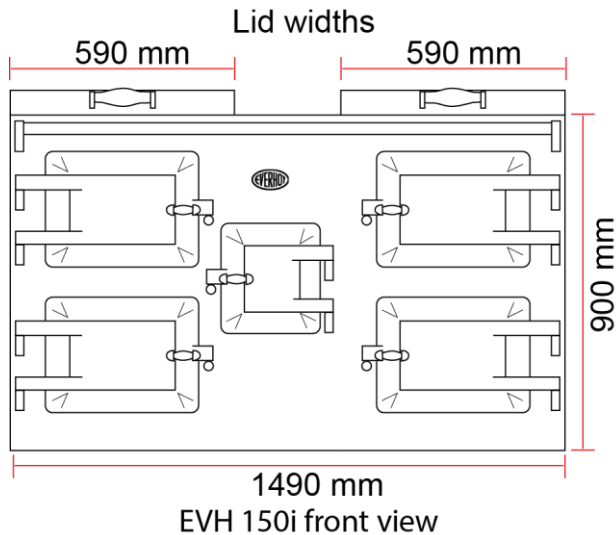
EVH150i dimensions
