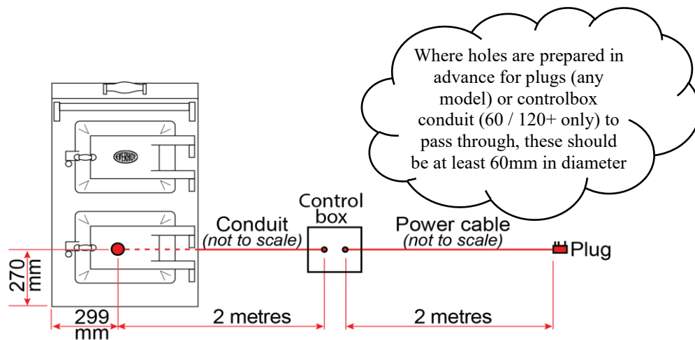
EVH 60 cable lengths
