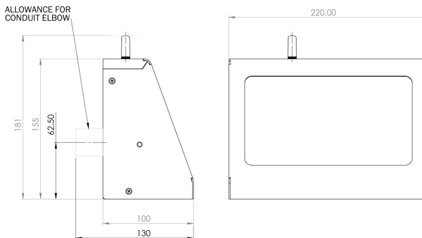
Controlbox and antenna dimensions
