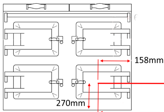
EVH 110+ cable lengths
