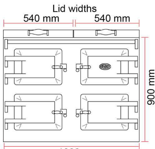
EVH 110+ front view
