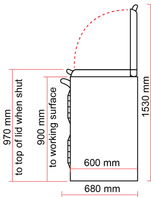
EVH 110+ side view
