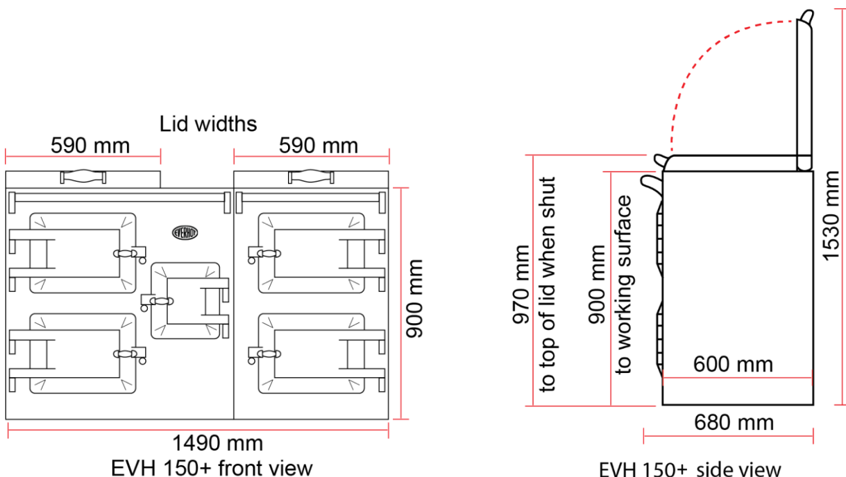
EVH150+ dimensions
