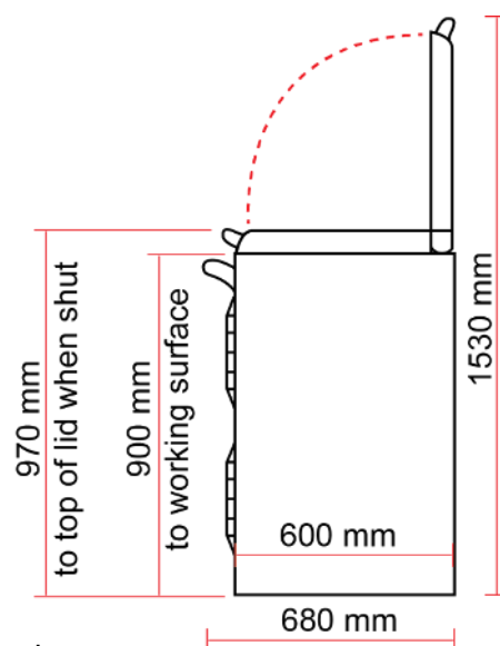
EVH 160i Side View
